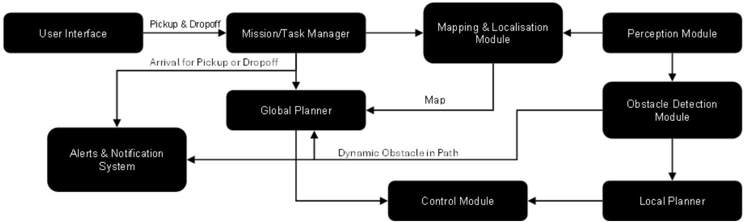
Figure 4.1 Block diagram representing the software architecture the system and their interactions at a high level
