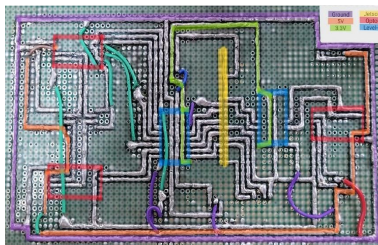
Figure 3.24 Photograph showing the underside of the completed perf board PCB showing the power lines
