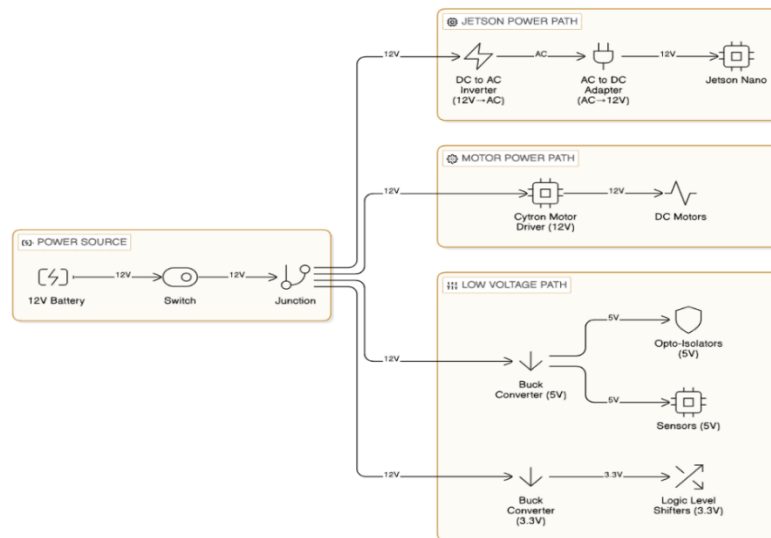
Figure 3.20 Block diagram of the power distribution architecture showing the battery, each regulated branch, and the loads supplied by each branch
