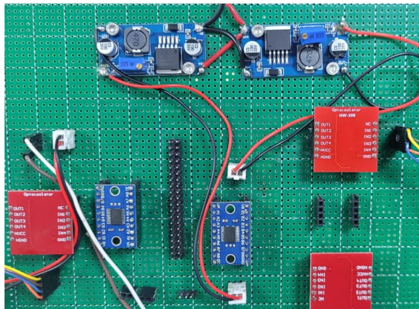
Figure 3.23 Photograph of the completed perf-board PCB showing the components, wire jumpers, and ribbon cable connector's header
