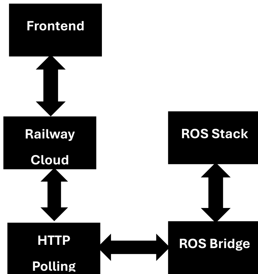
Figure 6.1: UI architecture
